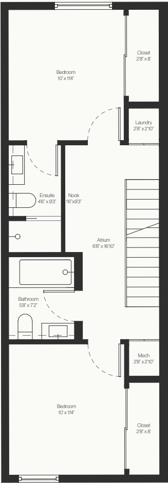
Level 3 574 sf
